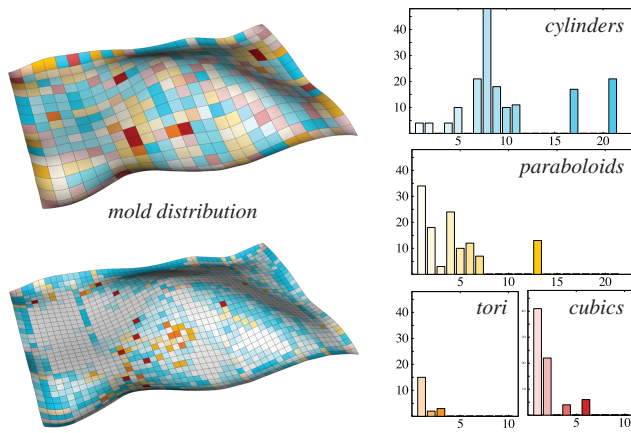
Figure 11: Distribution of panel types and mold reuse for two different refinement levels of the curve network. The histograms on the right illustrate mold reuse for the top image, where the x-axis denotes how many panels can be produced by a mold and the y-axis indicates the number of panels corresponding to these molds. (Mario Bellini Architects, Rudy Ricciotti, Museum of Islamic Arts at Louvre Museum, Paris.)
