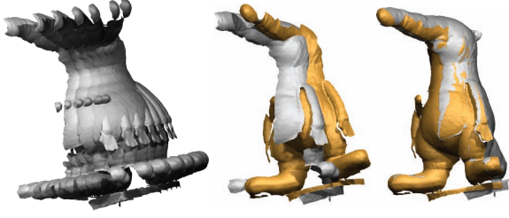
Figure 8: Accumulation Error. (Left) 300 scans of the coati model were registered (adjacent) pairwise, and the computed transforms were used to align the last frame to the first frame. Dynamic registration (right) gives good alignment, while ICP algorithm results in accumulation error (center). In presence of sufficient time sampling, our method does not need global error distribution.
