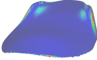
Figure 16: Visualization of Gaussian curvature of the design shown by Figures 11, 12. Blue corresponds to zero, red to the maximum value -0.02 (this means \rho = 7.07 ). The bounding box diagonal of this object is 188.
