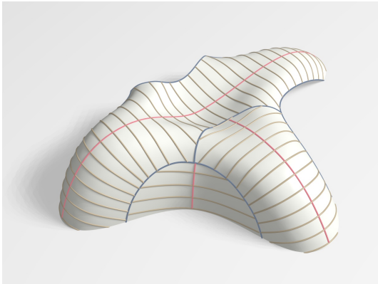
Figure 4: Designing a sequence of geodesics by choosing the locus (red) of minimum distance or maximum distance between neighbours. This is done by the parallel transport method . In this particular example, the method is applied not to the entire surface, but to previously selected patches.
