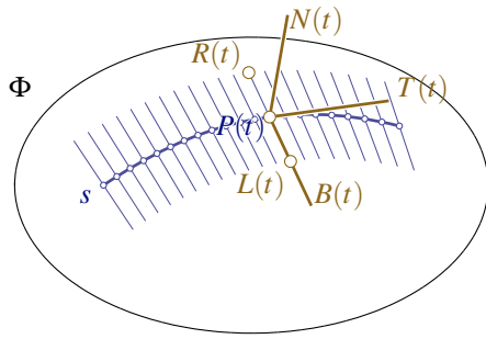
Figure 15: The binormal method defines a ruled panel surface from a central geodesic s via its Frenet frame T, N, B : The ruling passing through the central point P(t) on the geodesic is indicated by the binormal vector B(t) . The endpoints of the ruling segment are points L(t) and R(t) whose distance from P(t) is half the intended panel width.
