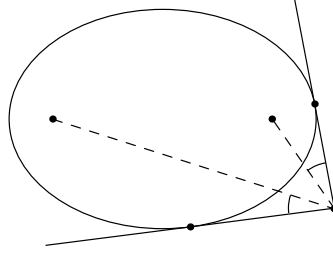
FIGURE 11: The angles between the tangent directions and the directions to the focal points of an ellipse are equal.
