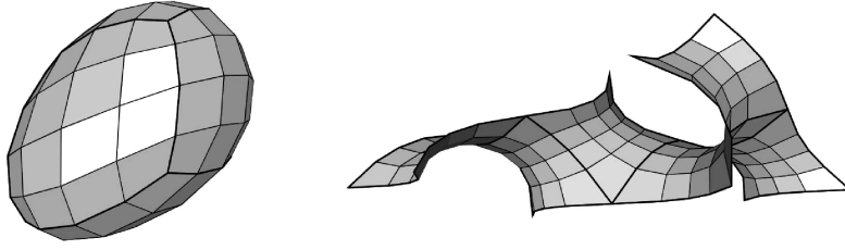
FIGURE 4: Discrete Koenigs nets interpreted as a Gauss image s , and its Christoffel dual minimal net m = s^* (courtesy P. Schröder).
