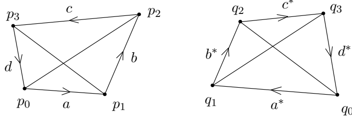
FIGURE 3: Dual quadrilaterals.
