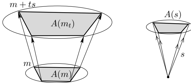
FIGURE 6: Parallel Q-nets m and m + ts with the unit Gauss map s . All the nets are circular. The pair (m, s) constitutes a principal contact element net.
