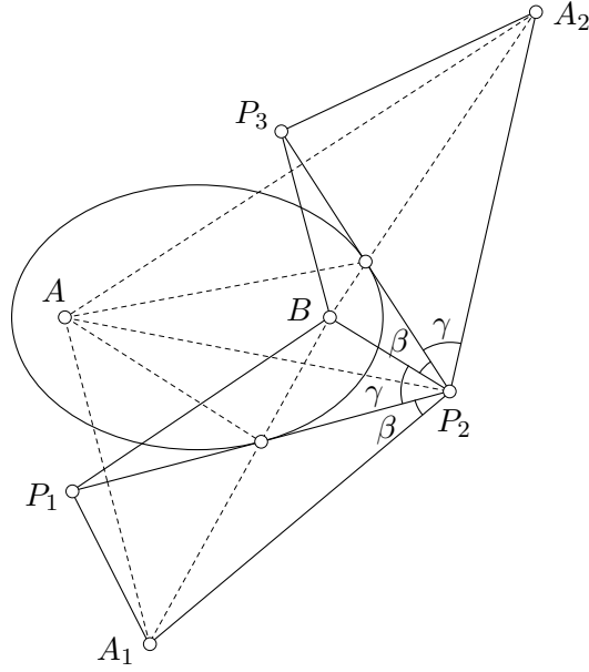
FIGURE 9: An external elliptic billiard. The trajectory \{P_i\}_{i \in \mathbb{Z}} is tangent to an ellipse.
