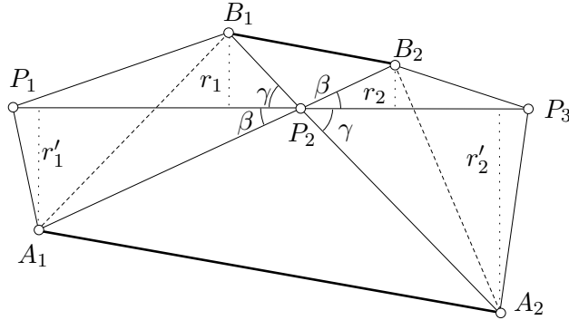
FIGURE 10: A discrete cmc surface with rotational symmetry generated from an elliptic billiard.
