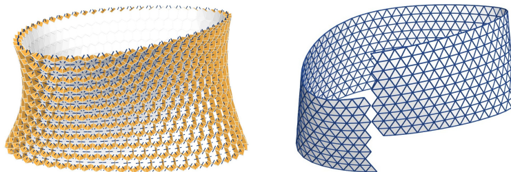
Figure 8: Lobel meshes and Honeycombs . A combinatorial dual to the walls of a honeycomb (left) is a triangle mesh where edges intersect at 60 degrees (right), implying the Lobel property. Step-by-step construction of the Lobel mesh orthogonal to the honeycomb is possible only for simply connected honeycombs; otherwise the construction does not globally close.
