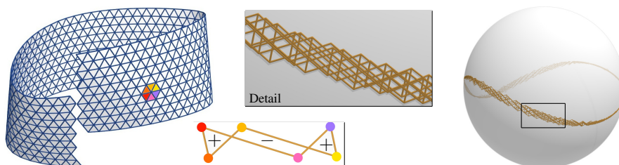
Figure 9: Local and global properties of Lobel meshes . The image at right illustrates the curve-like spherical image of the Lobel mesh at left. It follows from the discussion in [Jiang et al. 2014] that the normal vectors of a 1-ring neighbourhood of any vertex typically form a zero area hexagon on the unit sphere.
