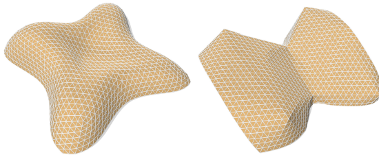
Figure 7: Projecting a triangle mesh onto the constraint space defined by the “Lobel” property makes all faces equilateral and the mesh developable, apart from cuts necessary to accommodate valence 5 vertices.
