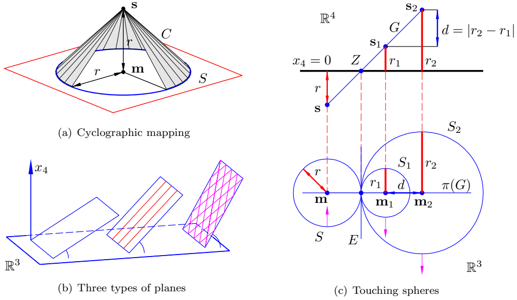
Fig. 1. Minkowski space and cyclographic mapping.
