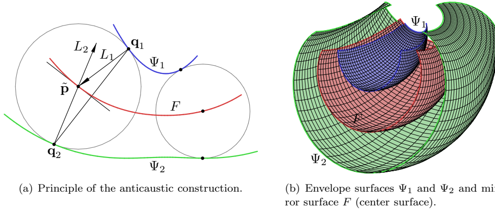
Fig. 3. Construction of an Anticaustic \Psi_2 with respect to illumination orthogonal to \Psi_1 and reflection at F .
