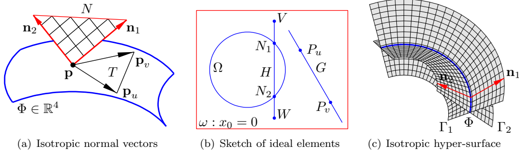
Fig. 2. Isotropic normals and isotropic hyper-surfaces.
