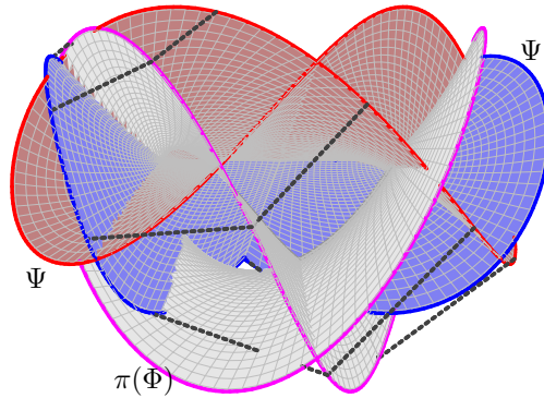
Fig. 6. Projection \pi(\Phi) of a surfaces of type 2 and envelope surface \Psi .
