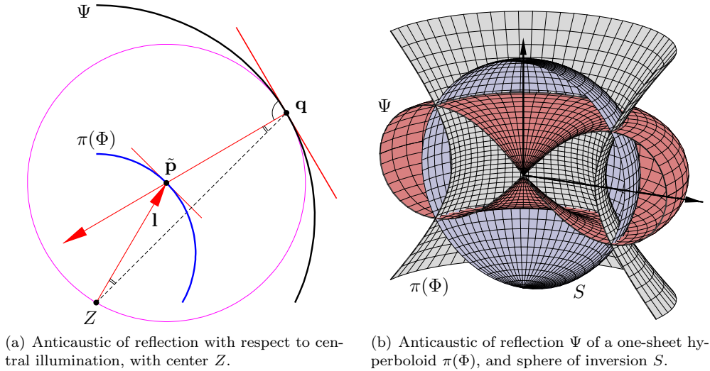
Fig. 5. Anticaustic construction and example.
