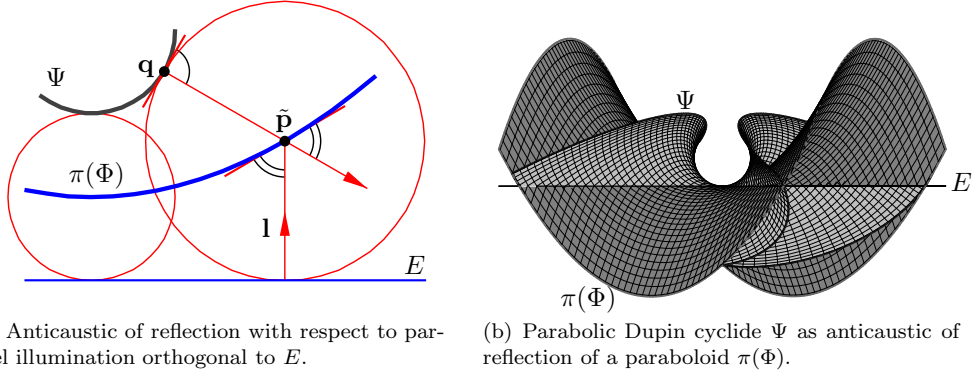
Fig. 4. Anticaustic construction and example.
