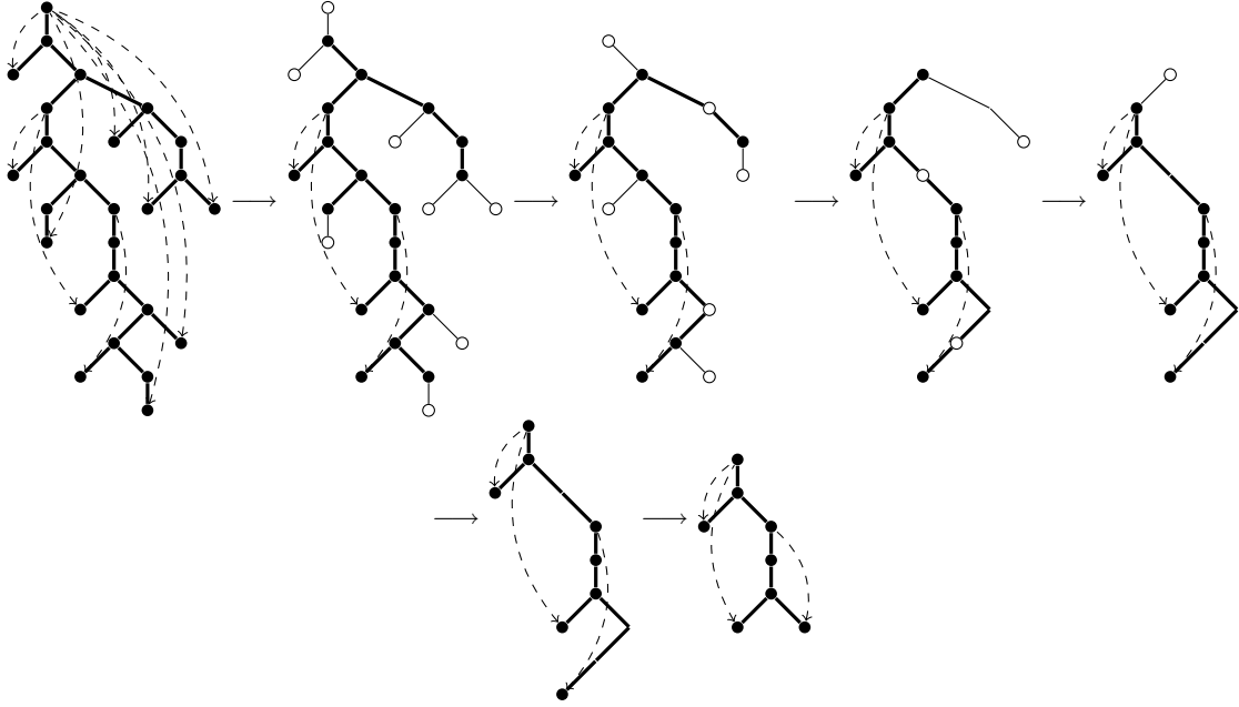
Figure 5: Finding the original closed lambda-term: first, the unary root node and all the leaves bound by the root are coloured white. Then delete the white nodes and colour all their neighbours white. Now continue recursively, where deletion of white unary nodes is done by removal and gluing the incident edges together.
