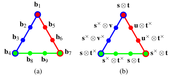
FIG. 4. (a) Subgraph of the triangle hypergraph depicted in Fig. 3 with a faithful orthogonal representation by decomposable vectors \mathbf{b}_2, \mathbf{b}_2, \dots, \mathbf{b}_6 and arbitrary vectors \mathbf{b}_1, \mathbf{b}_7, \mathbf{b}_8, \mathbf{b}_9 . Even though it turns out that \mathbf{b}_1 and \mathbf{b}_7 must be decomposable, the remaining vectors \mathbf{b}_8 and \mathbf{b}_9 have to be indecomposable. (b) An explicit example of a non-faithful orthogonal representation of the triangle hypergraph with only decomposable vectors resulting in the multiple occurrence of \mathbf{s} \otimes \mathbf{t} .
