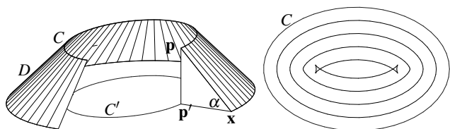
Figure 1: Left: Developable surface through an ellipse C , evaluation of the distance function of C' at x . Right: Ellipse with untrimmed interior offset curves.
