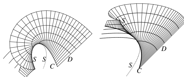
Figure 4: Developable surface D through a space curve C . The singular curve S (curve of regression) is displayed in dotted linestyle. Generating lines and level curves are shown.
