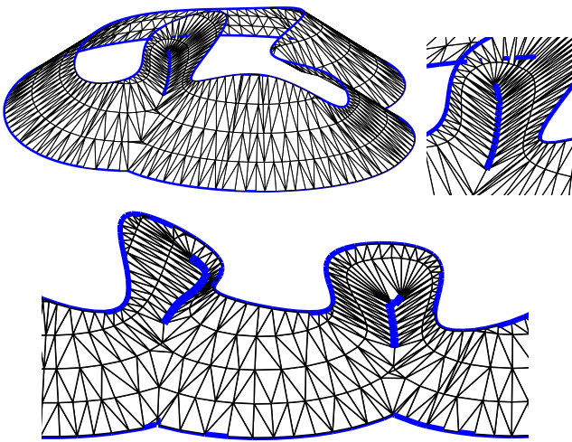
Figure 13: Self intersections of developable surfaces
